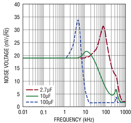
1.25V Output Voltage Noise Spectrum
